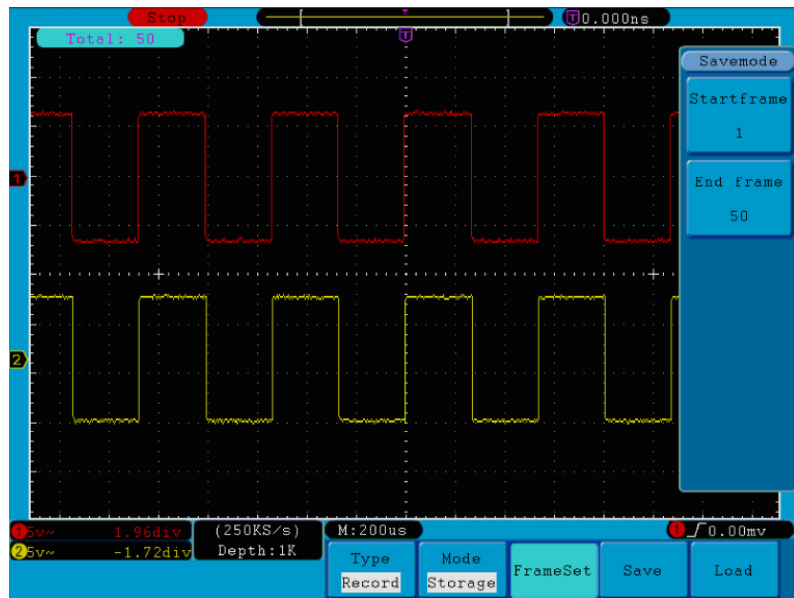
Fig. 51 Wave Storage
