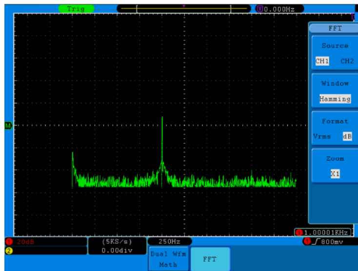
Fig. 21 Hamming window
