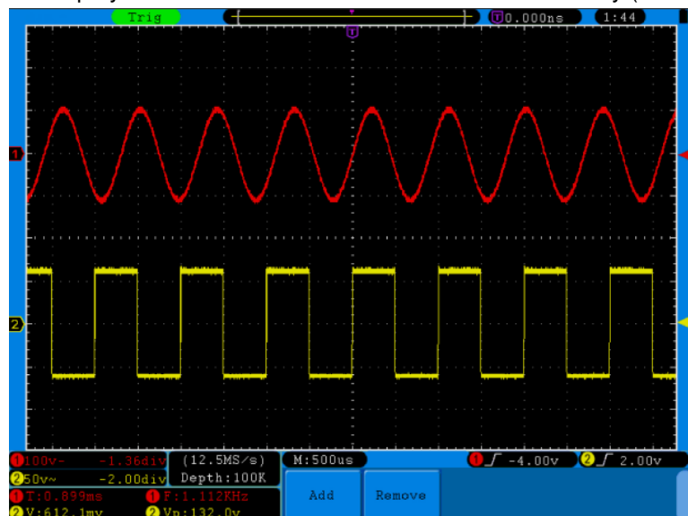
Fig. 67 automatic measurement
