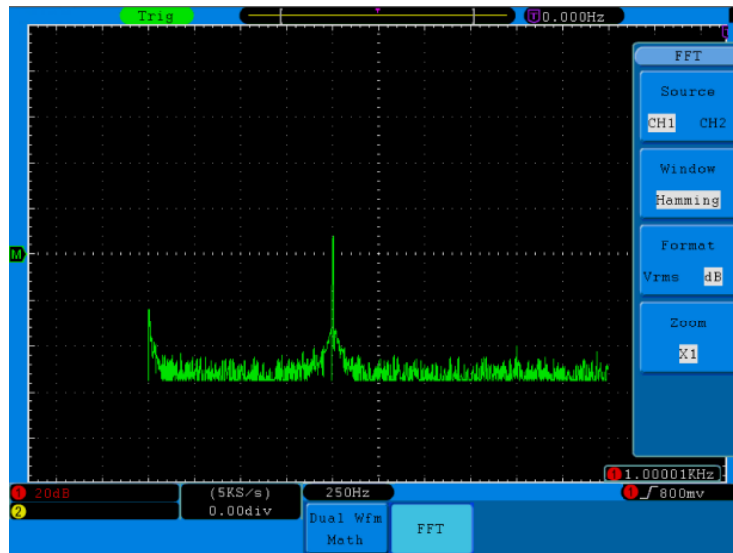
Abb. 21 Hamming-Fenster
