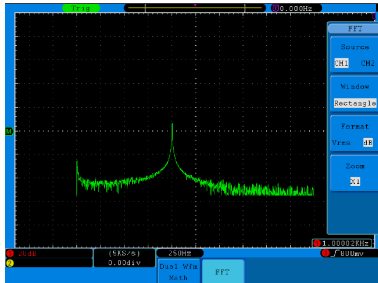
Fig. 21 Rectangle window
