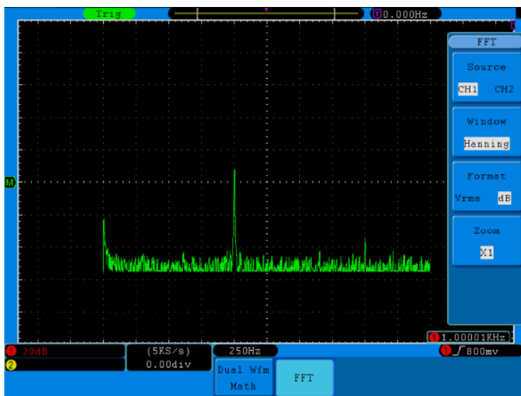
Fig. 23 Hanning window
