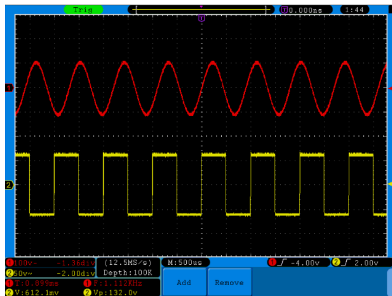
Abb. 68 automatic measurement
